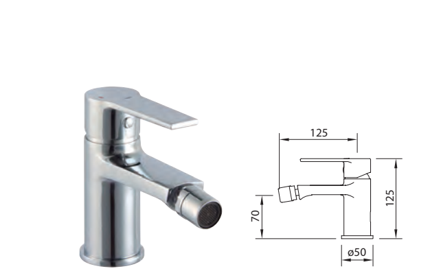
Mezclador con aireador a rótula, flexibles M-10 3/8" x 420 mm. Mixer, swivel aerator, flexible hoses M-10 3/8" x 420 mm. Mitigeur bidet, aérateur, raccords flexibles M-10 3/8" x 420 mm
