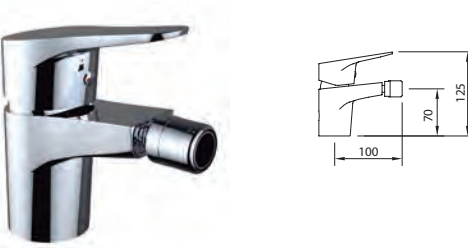
Mezclador con aireador a rótula, flexibles M-10 3/8" x 370 mm. Mixer, swivel aerator, flexible hoses M-10 3/8" x 370 mm. Mitigeur bidet, aérateur rotule, raccords flexibles M-10 3/8" x 370 mm
