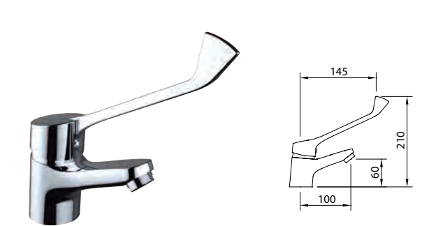
Mezclador con aireador, con palanca gerontológica y flexibles M-10 3/8" x 370 mm. Mixer with medical lever operated with aerator, flexible hoses M-10 3/8" x 370 mm. Mitigeur lavabo, manette médicale, aérateur, raccords flexibles M-10 3/8" x 370 mm
