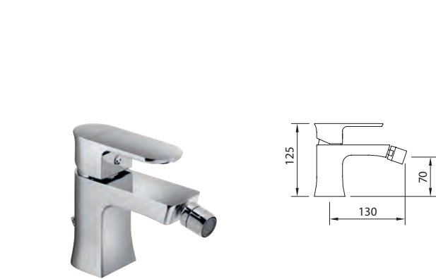
Mezclador con aireador a rótula, flexibles M-10 3/8" x 370 mm. Mixer, swivel aerator, flexible hoses M-10 3/8" x 370 mm. Mitigeur bidet, aérateur rotule, raccords flexibles M-10 3/8" x 370 mm
