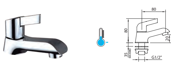
GRIFO SIMPLE REPISA 20 Single handle washbain tap 20 / Robinet simple 20
