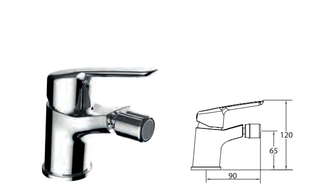
Mezclador con aireador a rótula, flexibles M-10 3/8" x 420 mm. Mixer, swivel aerator, flexible hoses M-10 3/8" x 420 mm. Mitigeur bidet, aérateur, raccords flexibles M-10 3/8" x 420 mm
